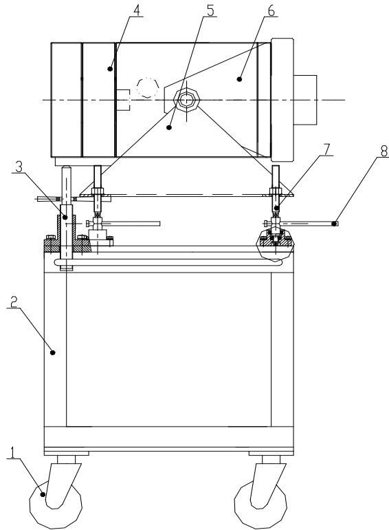
Die support cart
